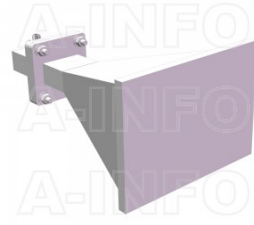
LB-112-15-C-3.5SPO Standard Gain Horn Antenna 7.05-10GHz 15dB Gain 3.5mm Female
