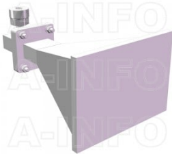
LB-112-15-C-7SPO Standard Gain Horn Antenna 7.05-10GHz 15dB Gain 7mm Female
